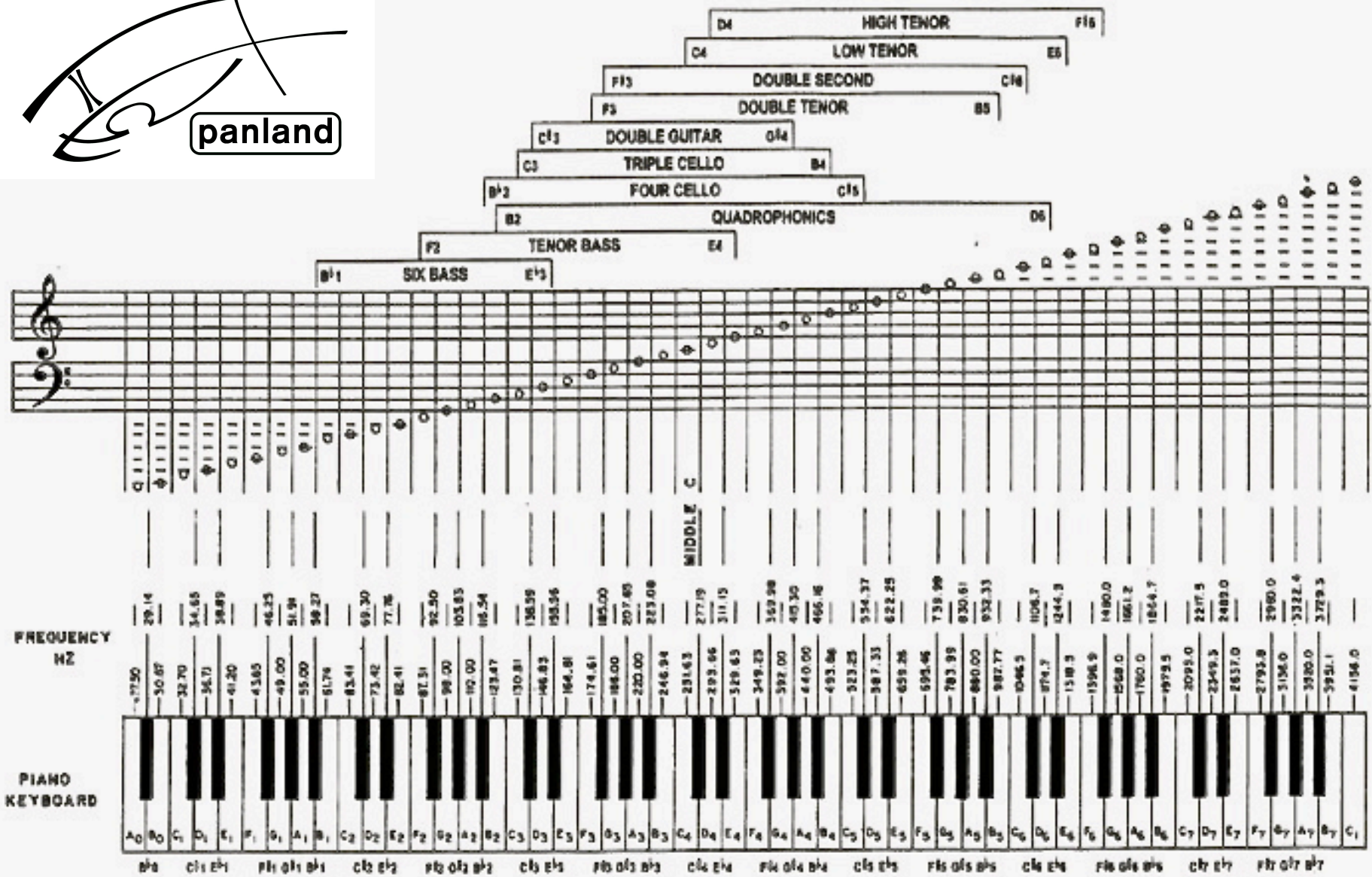
Chart showing the frequency range of the various members of the steel pan family
